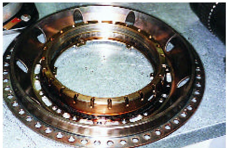
CF6-80C2B1F Number 5 Bearing Housing Mobil Jet Oil II: 13,700 hours, 2,200 cycles Minimal deposits with Mobil Jet Oil II.
